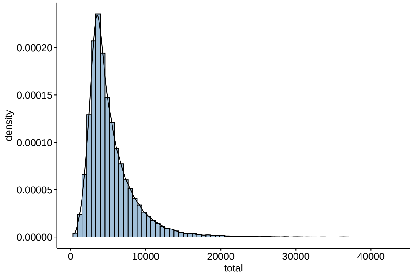
Cluster 0
